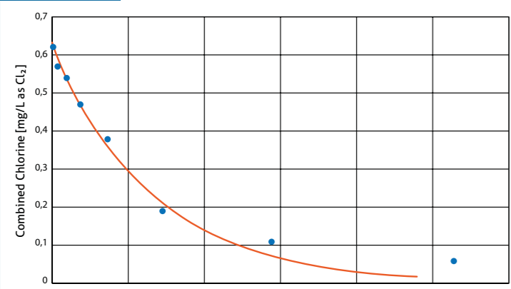
Figure 1 Measured and modelled photolysis of a specific organic chloramine with an Ultraaqua 3kW medium pressure UV reactor.
